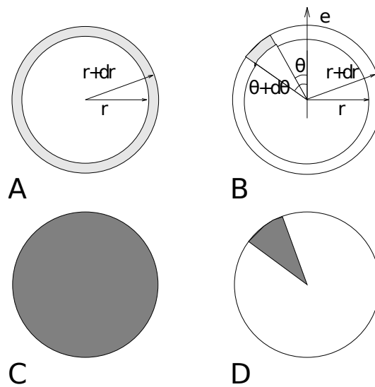
Fig. 5.50: Definition of slices in gmx rdf (page 133): A. g_{AB}(r) . B. g_{AB}(r, \theta) . The slices are colored gray. C. Normalization \langle \rho_B \rangle_{local} . D. Normalization \langle \rho_B \rangle_{local, \theta} . Normalization volumes are colored gray.
